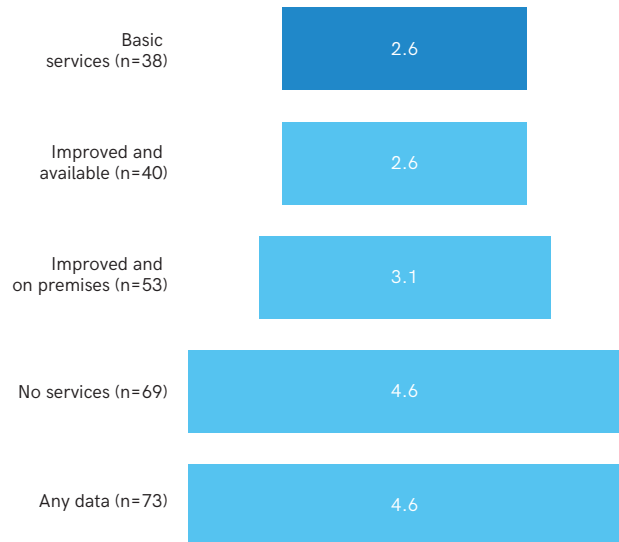
FIGURE 15 Data coverage for water services in health care facilities, by indicator, number of countries and population with data available (billions), 2016
